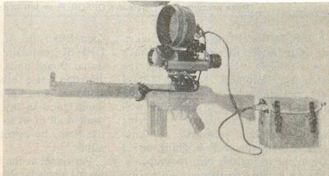
W. German Eltro B8-V Infrared (active) sight on G-3.
